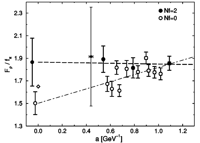
FIG. 40. Ratio of pseudoscalar and vector decay constants in full and quenched QCD.
